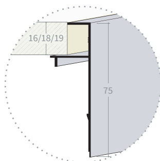
FBS7518 (pannelli da panels from 18 - 19 mm) FBS7515 (pannelli da panels from 16 mm)
