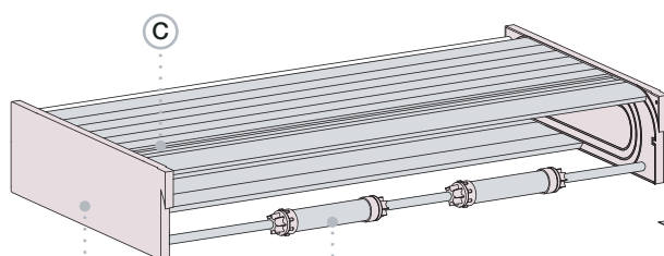
FBS9208 pista coiler
