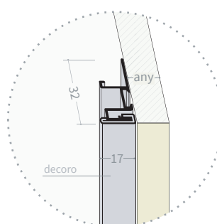
FBS7554 + FBS2063 (decoro decor)
