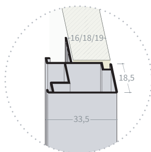
FBS7519 (pannelli da panels from 18 - 19 mm) FBS7516 (pannelli da panels from 16 mm)
