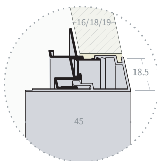
FBS7558 + FBS7555 (decoro decor ) (pannelli da panels from 18/19 mm) FBS7551 + FBS7555 (decoro decor ) (pannelli da panels from 16 mm)
