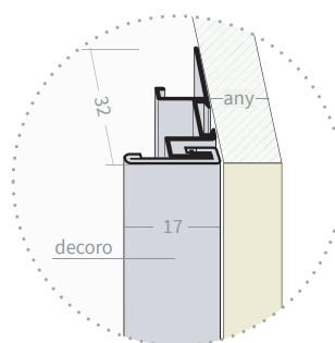
FBS7554 + FBS2062 (decoro decor )
