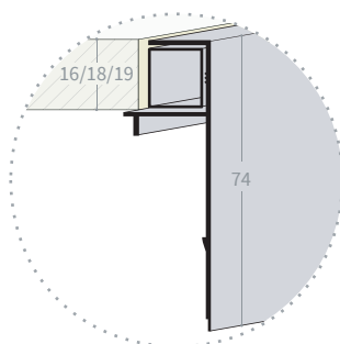
FBS7518 + FBS7553 (sottotop under top )
