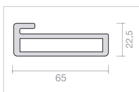
FBS 9444 per for FBS 3045 Flangia paraspigoli Safety flange
