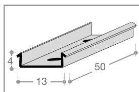
FBS2085 profilo base in alluminio SN aluminium fixing profile SN
