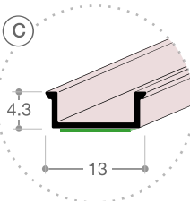
FBS6052 base in polistirene polystyrene base
