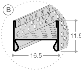
FBS2082 wind corpo body
