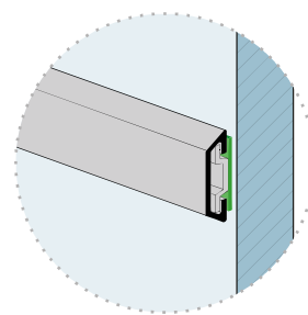
PROFILATI DECORATIVI DECORATIVE PROFILES
