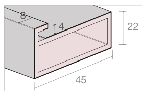
FBS 3045 Profilo perimetrale Frame profile
