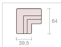
FBS 9445 per for FBS 3045 Angolo a scomparsa Concealed corner
