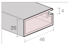
FBS 3046 Profilo perimetrale Frame profile
