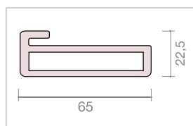
FBS 9444 per for FBS 3045 Flangia parasigoli Safety flange
