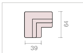
FBS 9446 per for FBS 3046 Angolo a scomparsa Concealed corner
