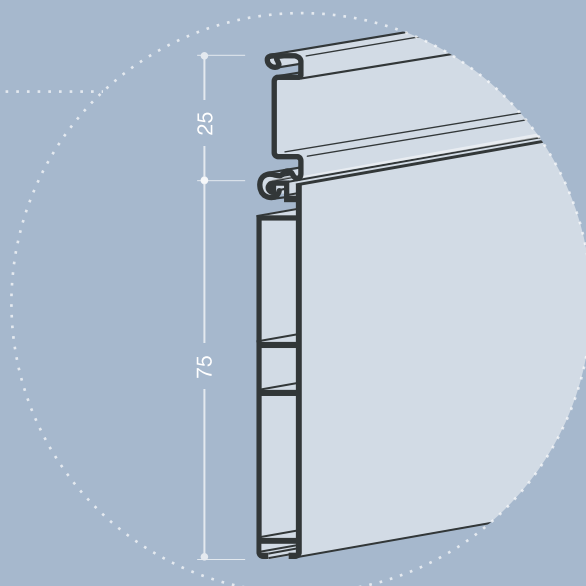
PROFILO CON MANIGLIA / PROFILE WITH HANDLE cod. FBS7512 + FBS2010 ( handle )
