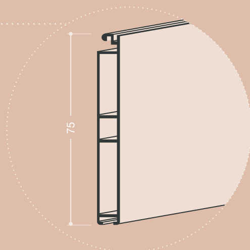
PROFILO TERMINE / BOTTOM PROFILE cod. FBS7512
