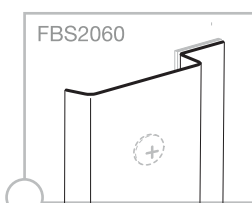
profilo copriviiti screw cover profile
