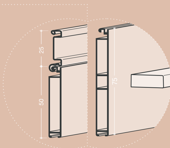
PROFILO CON MANIGLIA / PROFILE WITH HANDLE cod. FBS7547 + FBS2010 ( handle ) cod. FBS7512 + fbs7591 ( handle )
