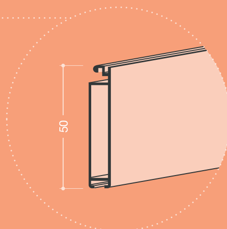
PROFILO TERMINALE / BOTTOM PROFILE cod. FBS7547
