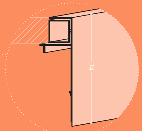
PROFILO TOP / TOP PROFILE cod. FBS7518 + FBS7553 ( sottotop )
